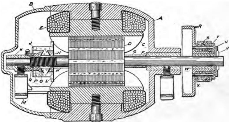
FIG. 170.—Sectional Diagram of the Apple Igniting Dynamo. The parts shown are: A, cast iron body containing the moving parts; B, the hinged lid of the body; C, the one pole piece of one of the field magnets; F, brass bearing of the armature spindle; G and H, fibre tubes surrounding the spindle; K, brass spider supporting the spindle; L, commutator; M, wick feed oil cup; N, beveled nut supporting the commutator; O, P, Q, supports of the commutator; R, the driving disc; S, lever friction pinion. This machine can generate a direct current at 8 volts at a speed of between 1,000 and 1,200 revolutions per minute. It is provided with a simple centrifugal governor that automatically interrupts the driving connections when a certain speed has been exceeded.
